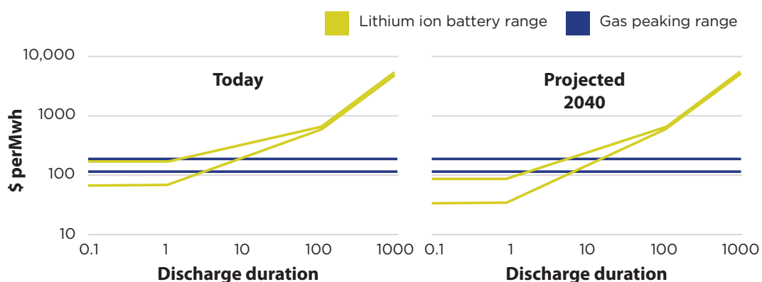
Figure 18: Comparison of storage technology costs
